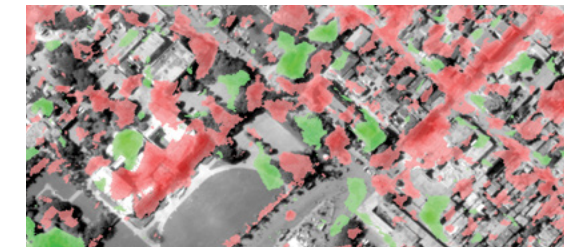
DSMs from stereo satellite imagery before and after the 2010 Haiti earthquake. Red shows areas of negative elevation change indicating earthquake damage. Stereo imagery from the DSM generation courtesy of DigitalGlobe® and GeoEye.
